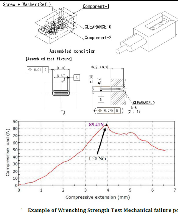
Example of Wrenching Strength Test Mechanical failure point
