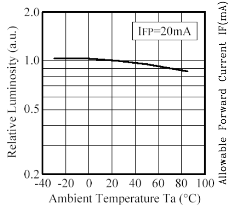
■ Ambient Temperature vs. Relative Luminosity
