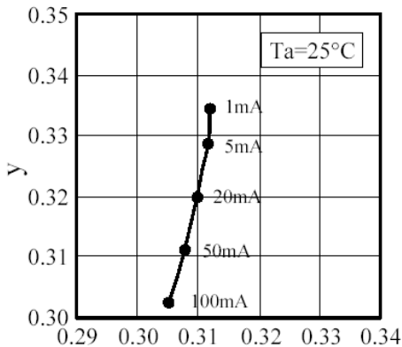
■ Forward Current vs. Chromaticity Coordinate
