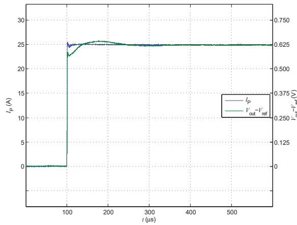
Figure 8: Step response
