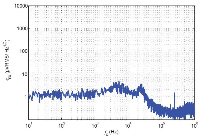
Figure 9: Output noise voltage spectral density
