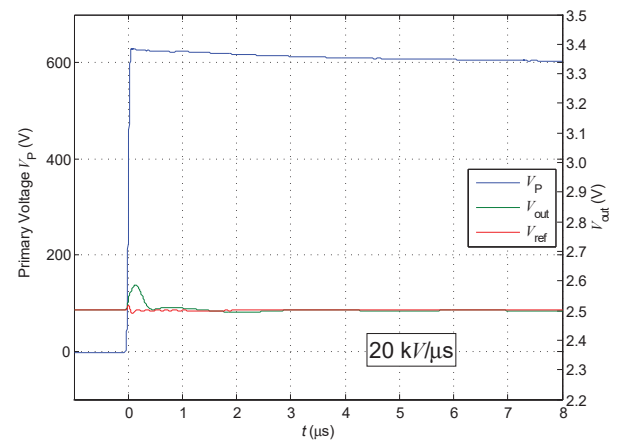
Figure 5: dv/dt
