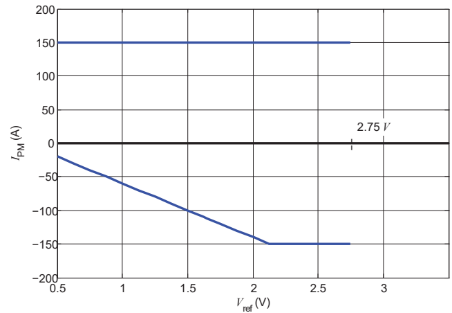
Figure 19: Measuring range versus external V_{ref} LESR 50-NP/SP1
