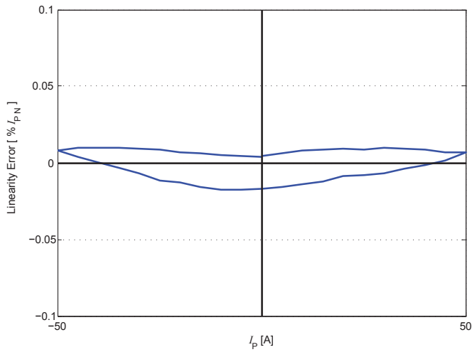
Figure 6: Linearity error
