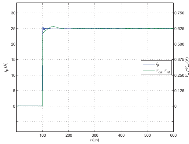
Figure 3: Step response
