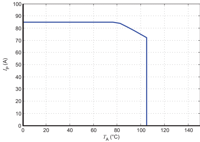
Figure 11: I_p vs T_A for LESR 25-NP/SP1
