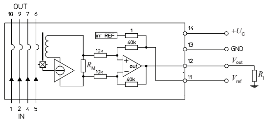
Figure 15: Test connection
