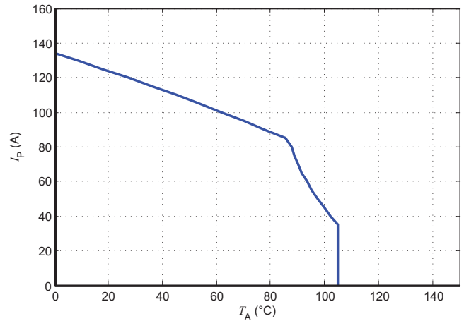
Figure 12: I_p vs T_A for LESR 50-NP/SP1
