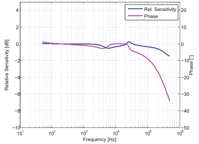
Figure 7: Frequency response
