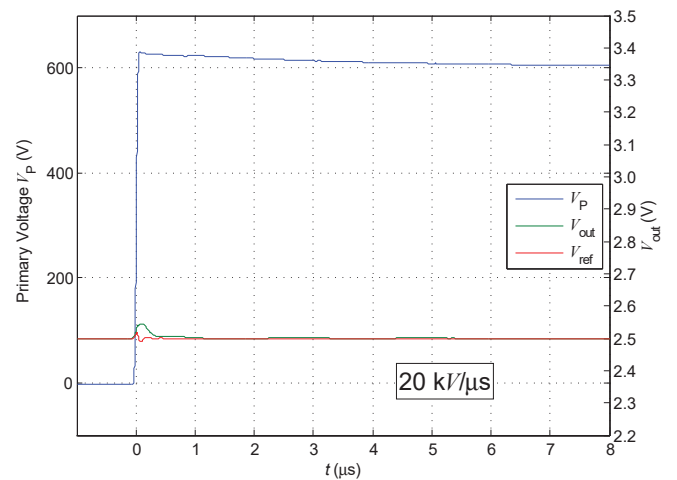
Figure 10: dv/dt
