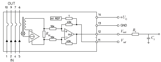
Figure 17: filtered V_{out} connection
