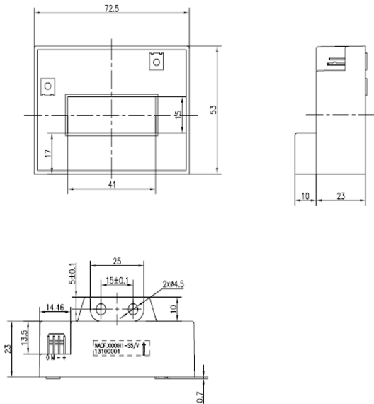
NACF.1000H1-S5/V 电压传感器外形图 Dimensions NACF.1000H1-S5/V Series (in mm)
